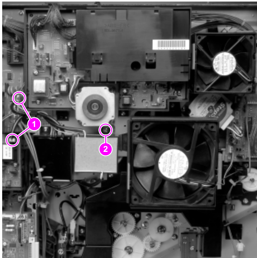
Figure 135. High-voltage converter 2
