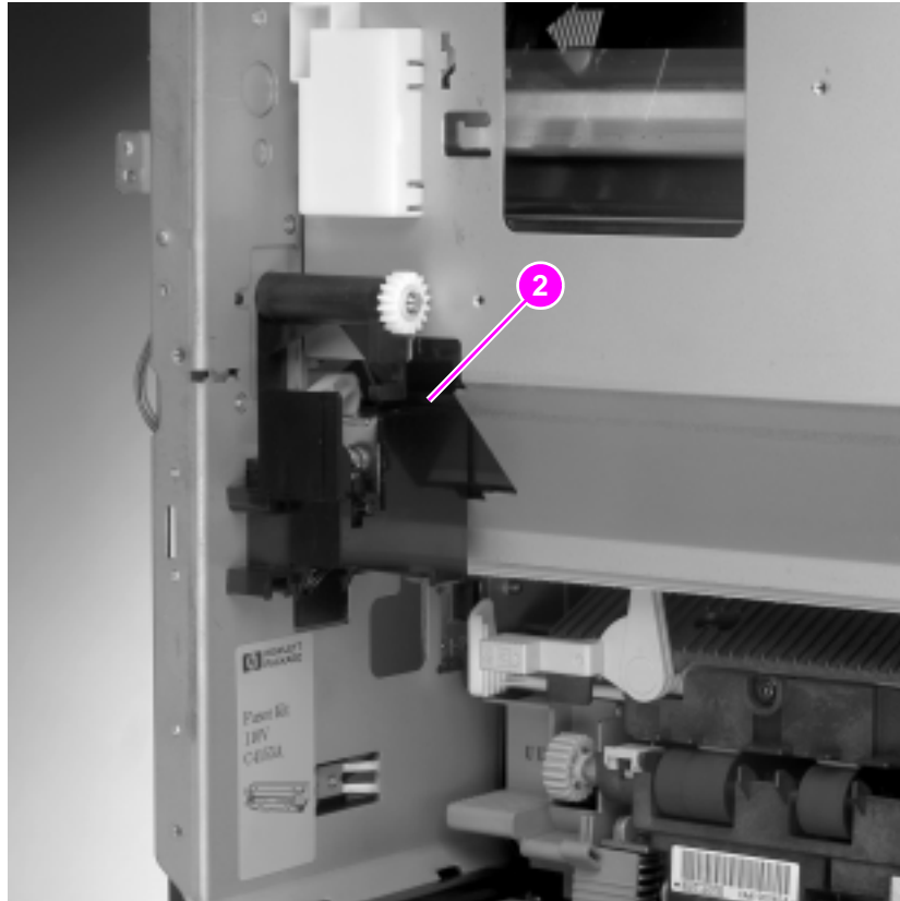
Figure 105. Face-up solenoid
