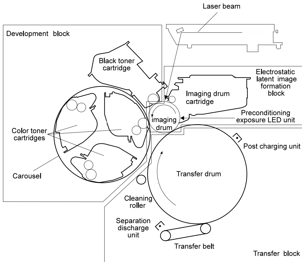
Figure 27. Image formation
