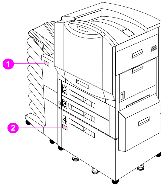
Figure 16. Paper handling accessory status LEDs
