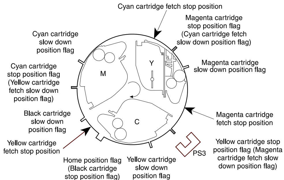
Figure 46. Carousel control
