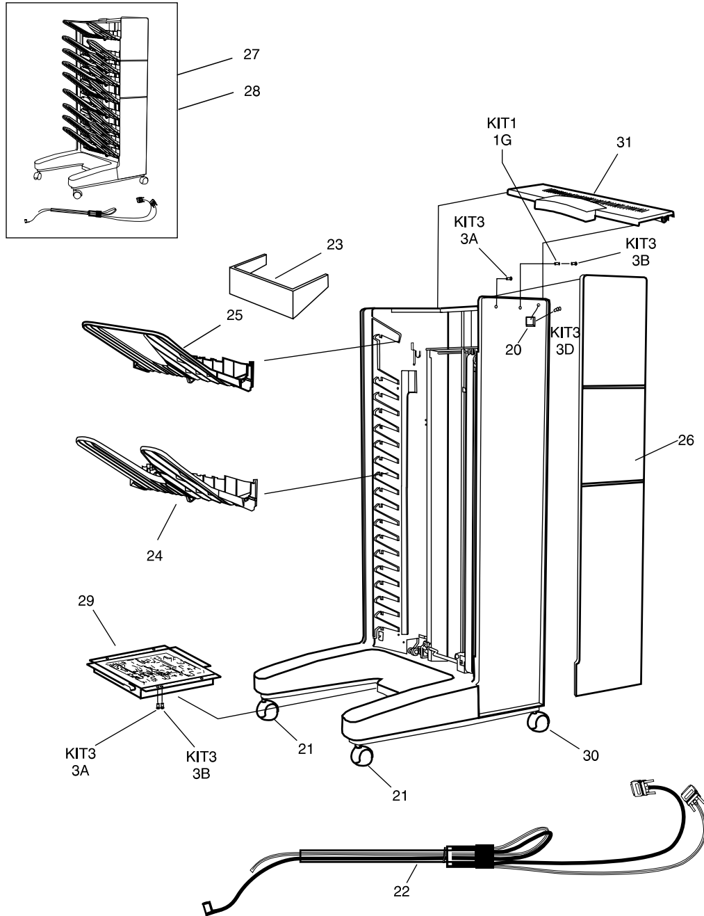
Figure 244. Multi-bin mailbox components (1 of 3)
