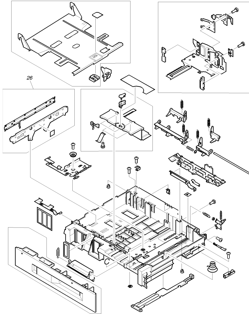
Figure 226. Tray 3 assembly
