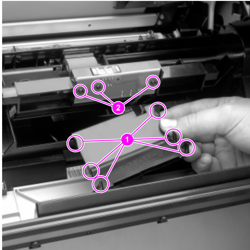
Figure 112. Density sensor
