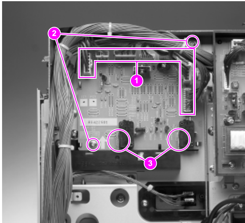
Figure 136. High-voltage converter 2
