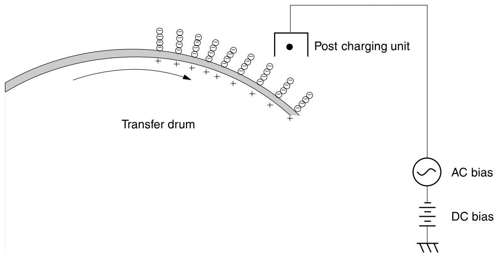
Figure 33. Post charging
