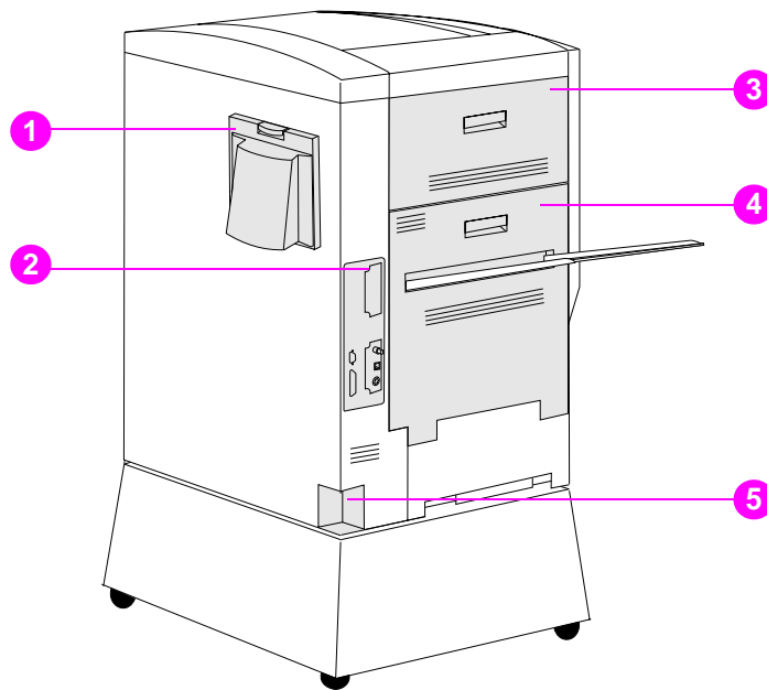
Figure 4. Rear view
