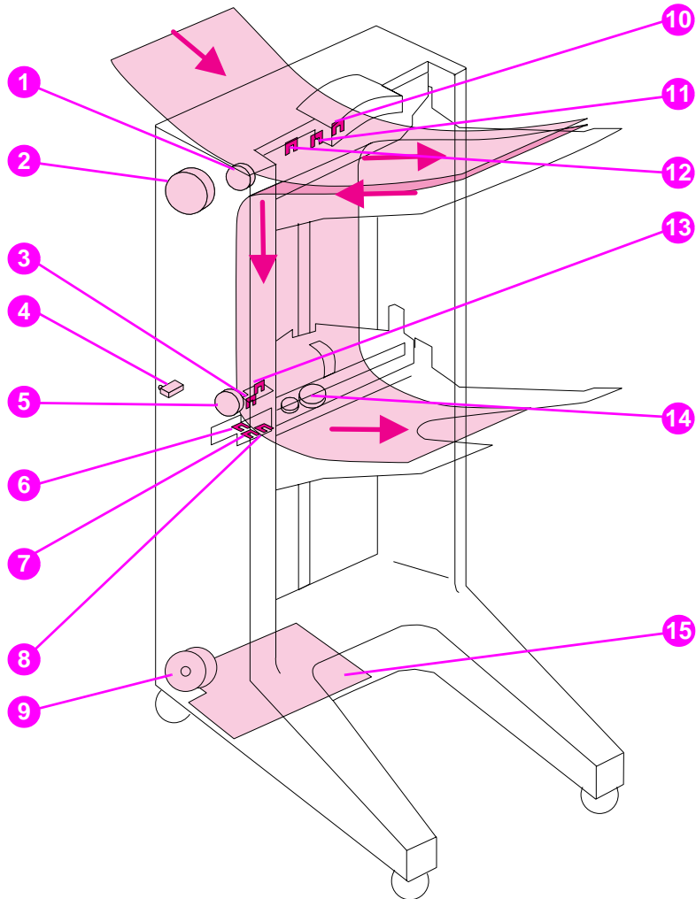
Figure 67. Multi-bin mailbox sensors
