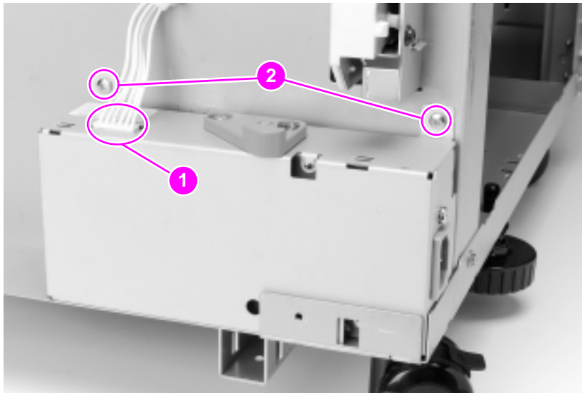
Figure 151. Power supply
