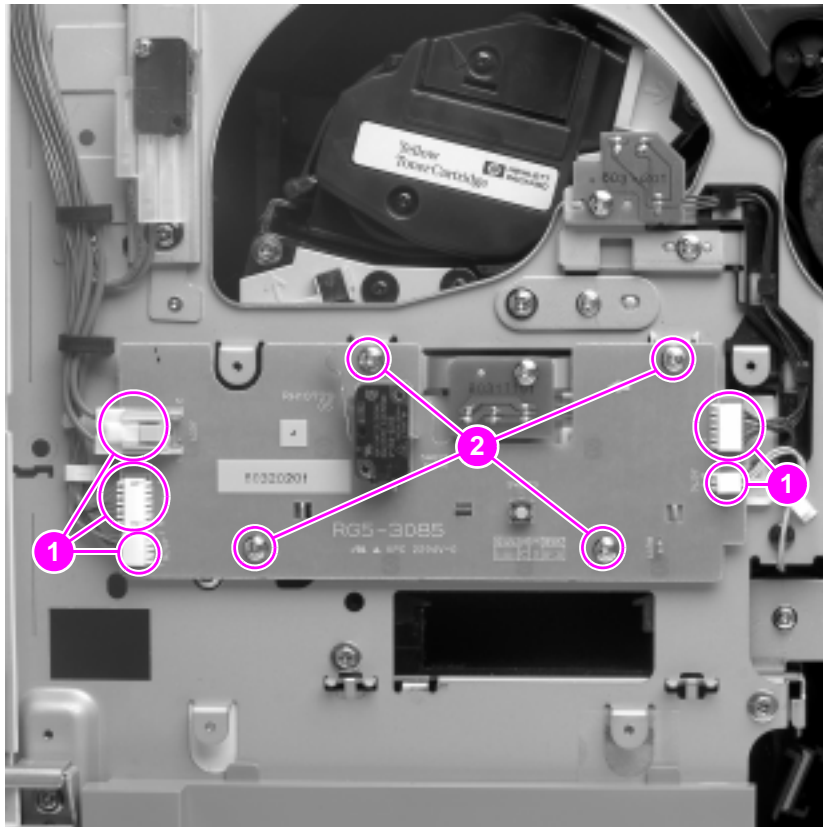
Figure 99. Subrelay PCA
