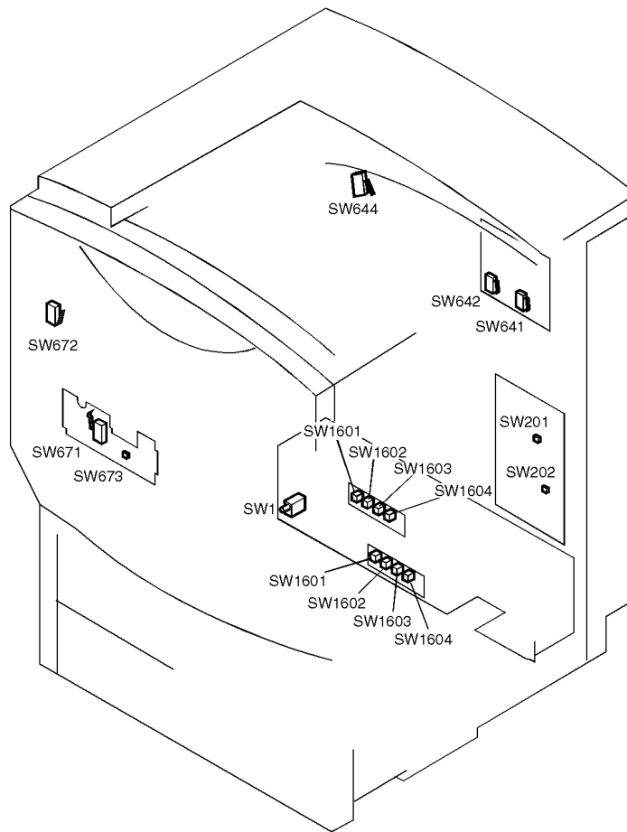
Figure 61. Printer switches
