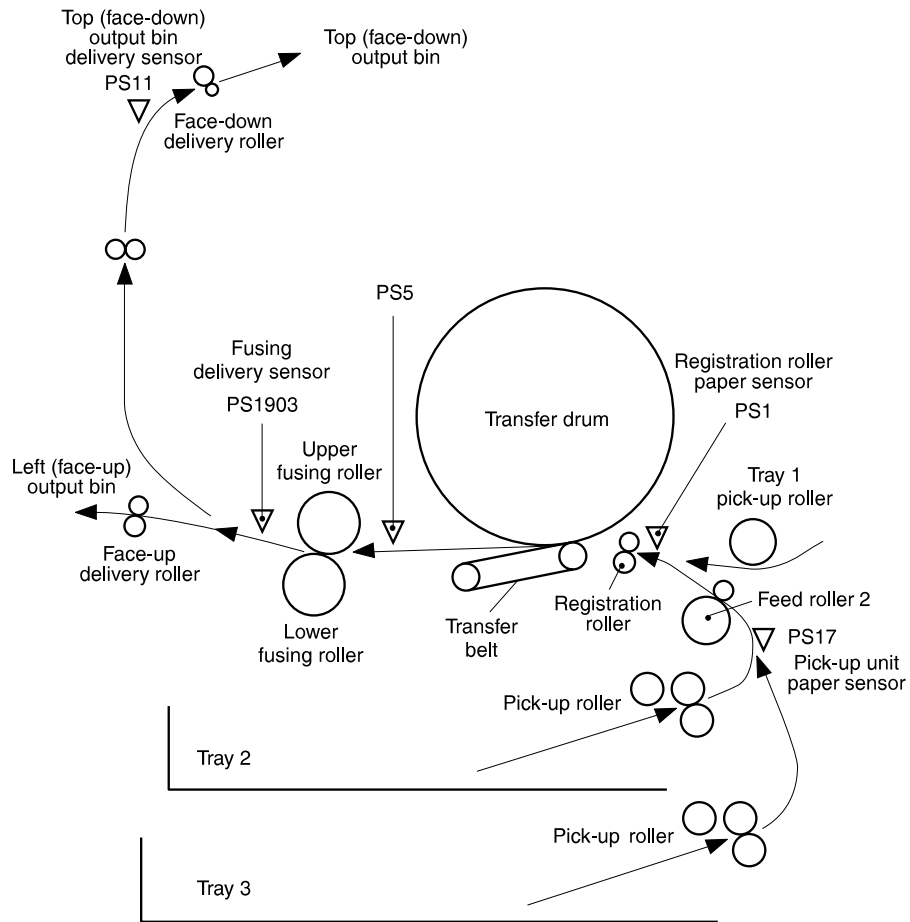
Figure 57. Paper path
