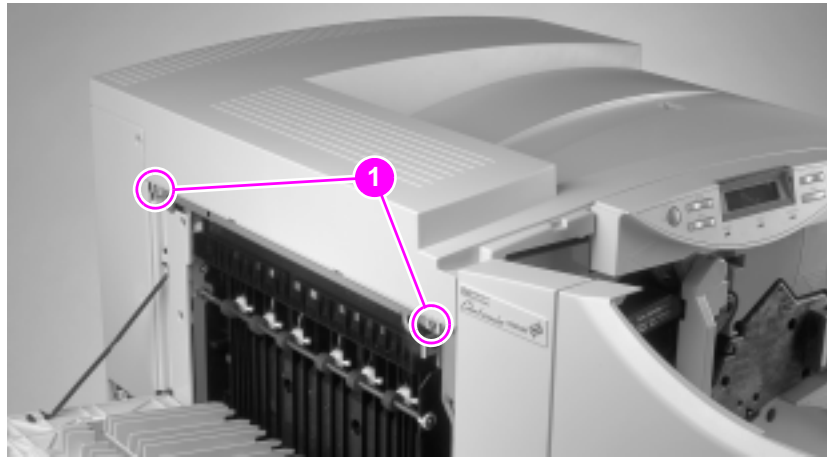
Figure 80. Screws behind left door
