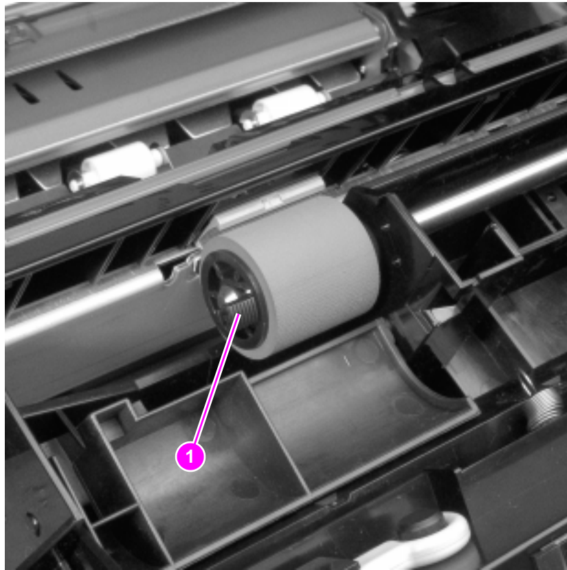
Figure 108. Pick-up roller
