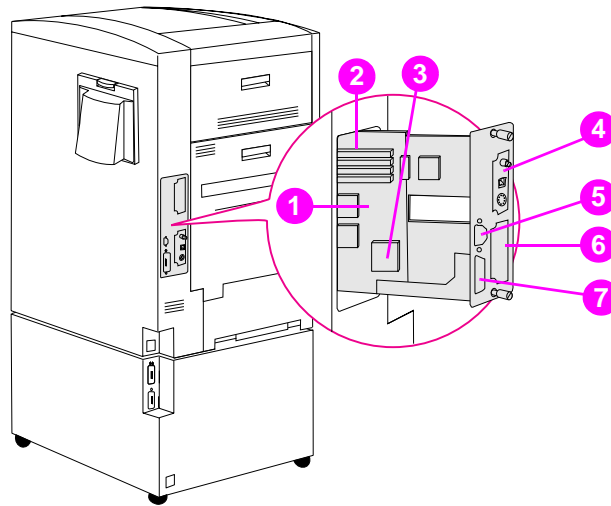
Figure 5. Formatter assemblies
