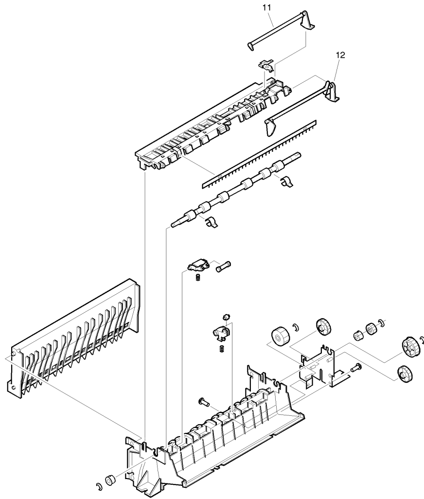
Figure 236. Delivery assembly
