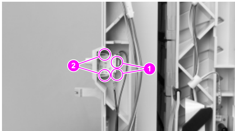
Figure 177. Interlock switch
