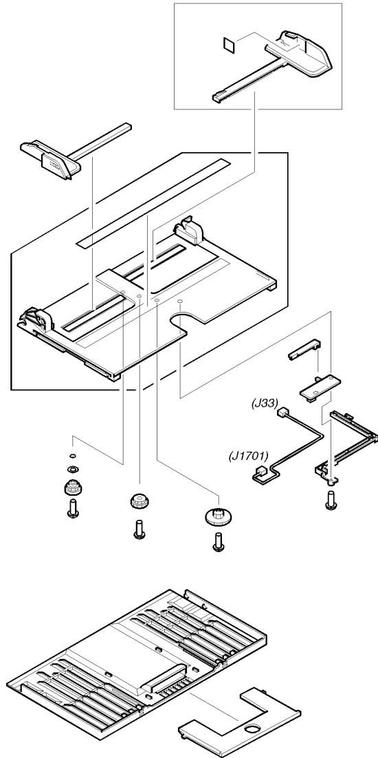
Figure 235. Tray 1 assembly
