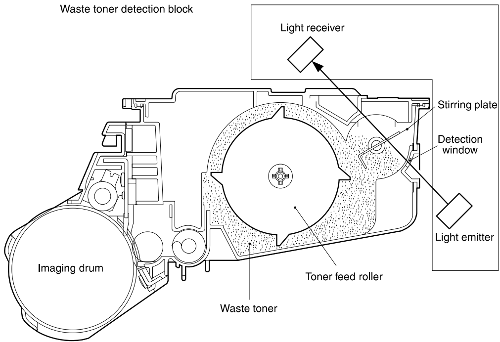
Figure 40. Waste toner level detection
