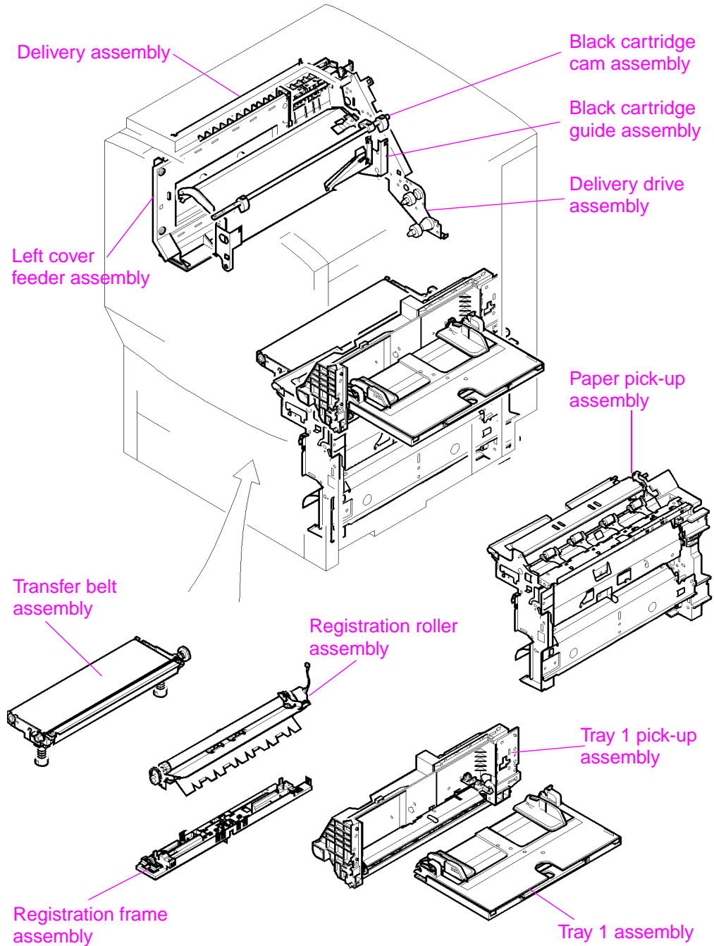
Figure 212. Major assembly locations (1 of 2)
