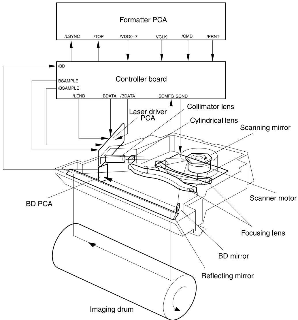
Figure 50. Laser/scanner
