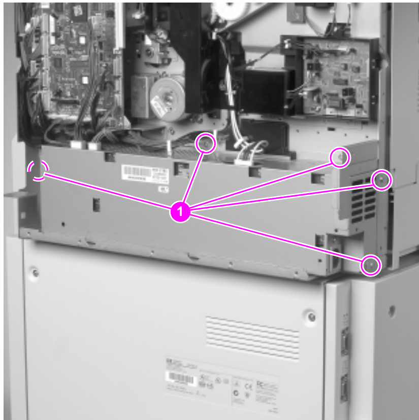
Figure 122. Power supply
