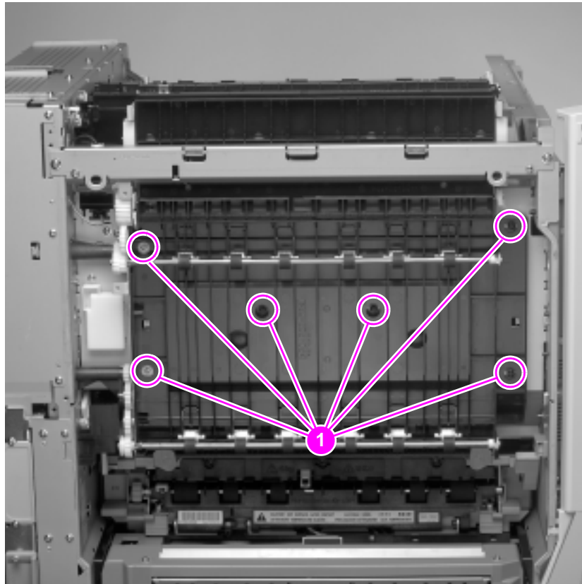
Figure 103. Feeder assembly
