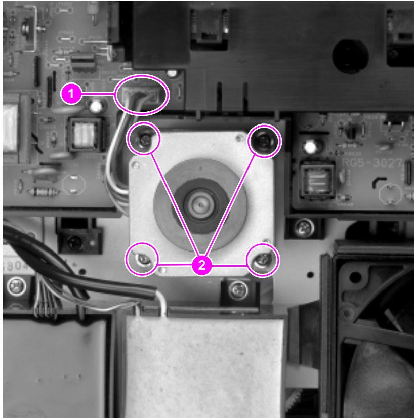
Figure 124. Cartridge motor
