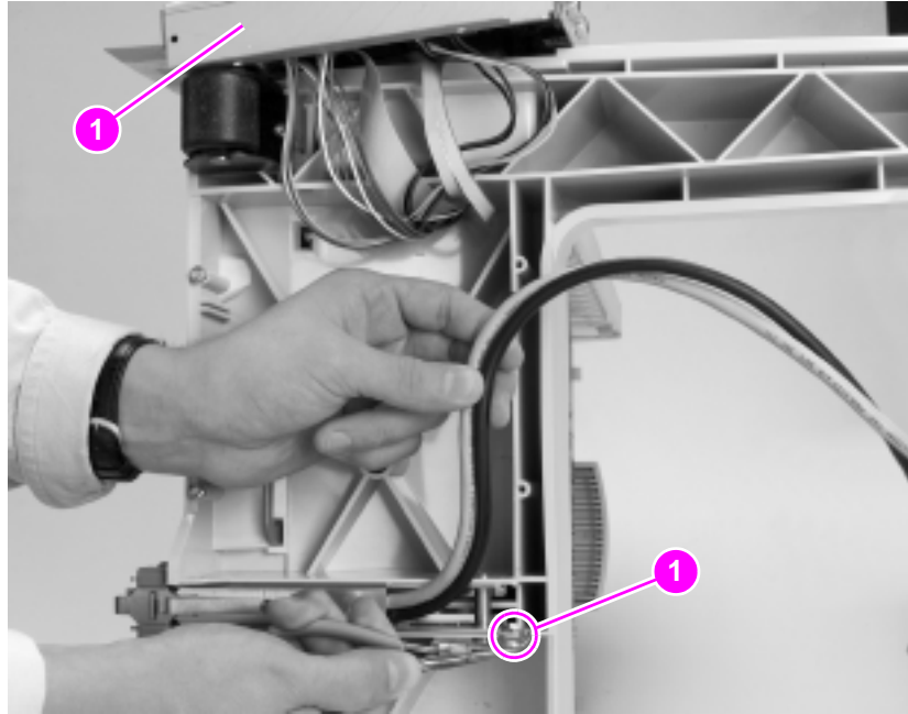
Figure 180. Attachment assembly
