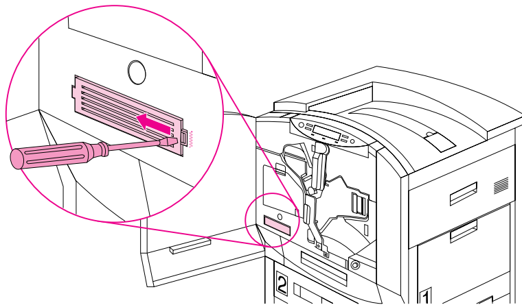
Figure 20. Removing the waste toner tray cover
