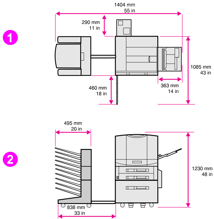
Figure 1. Space requirements
