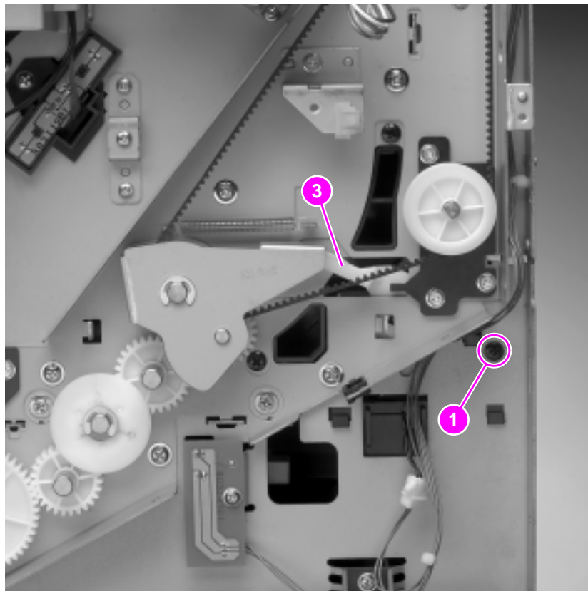
Figure 104. Face-up solenoid
