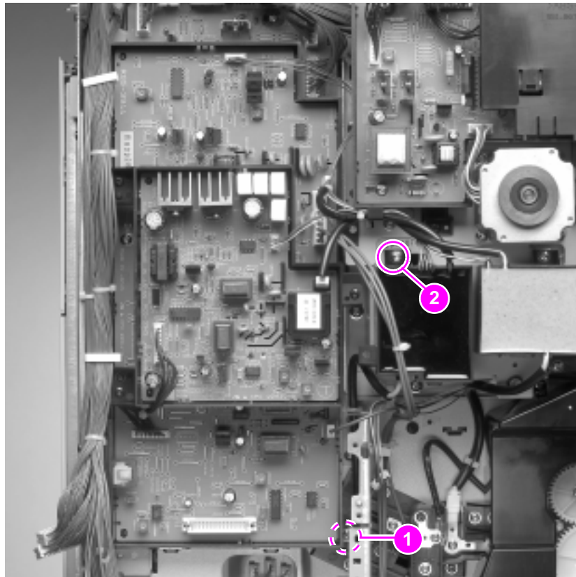
Figure 133. High-voltage converter 1
