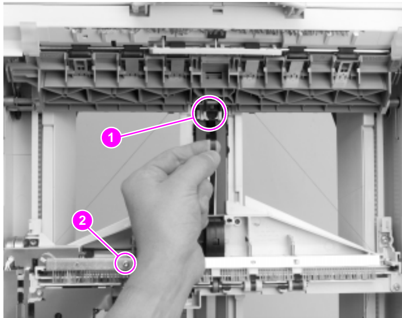
Figure 167. Metallic tape and housing assembly (1 of 2)
