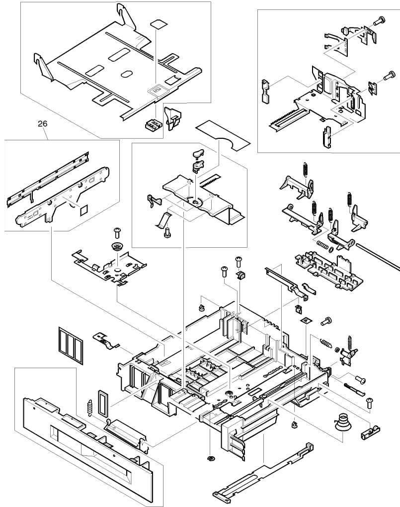
Figure 227. Tray 2 assembly
