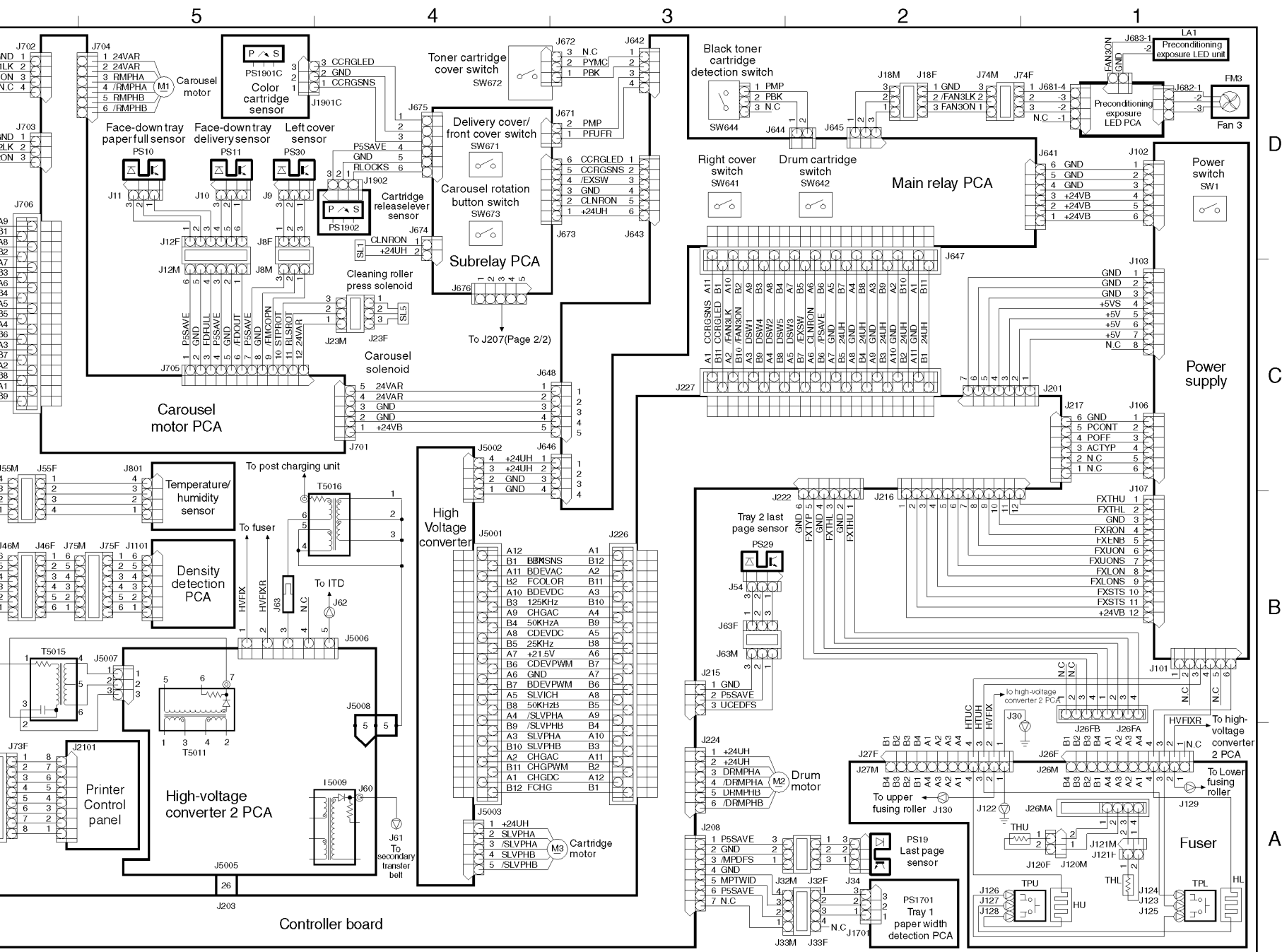
Printer circuit diagram (1 of 2)
