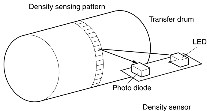
Figure 43. Density sensor
