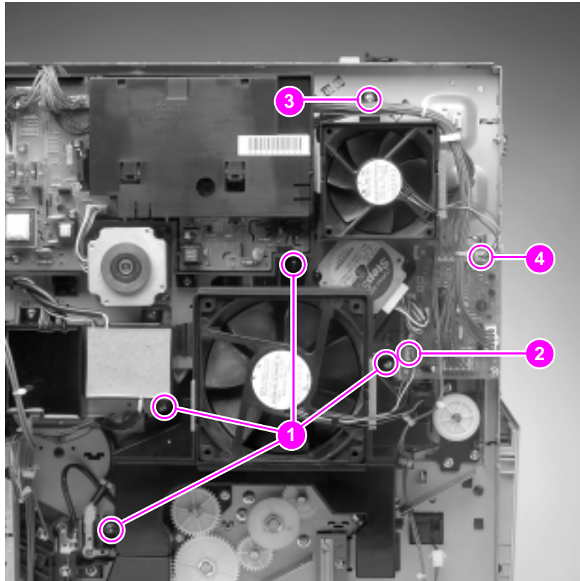
Figure 127. Fans 1 and 2 housing assemblies
