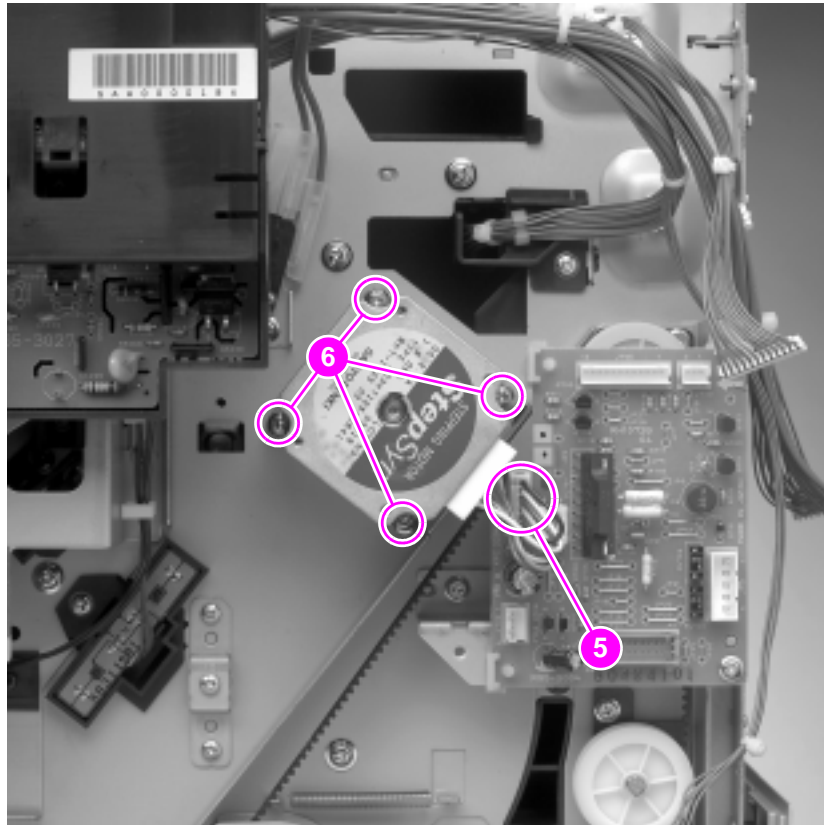
Figure 128. Carousel motor
