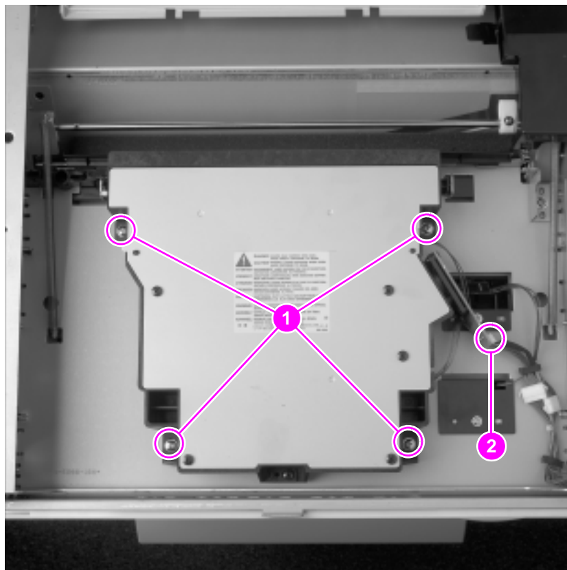
Figure 94. Scanner unit
