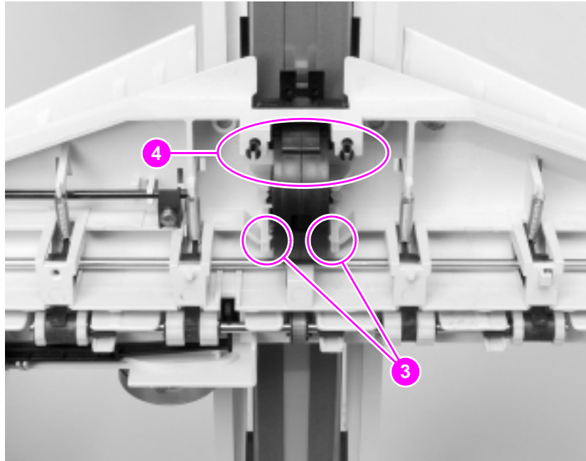
Figure 168. Metallic tape and housing assembly (2 of 2)
