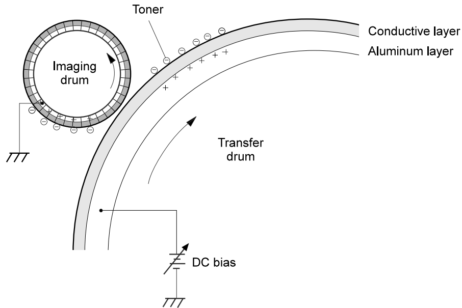
Figure 32. Primary transfer
