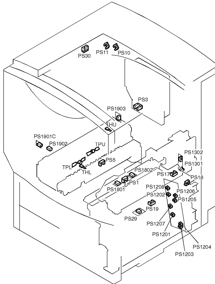
Figure 60. Printer sensors
