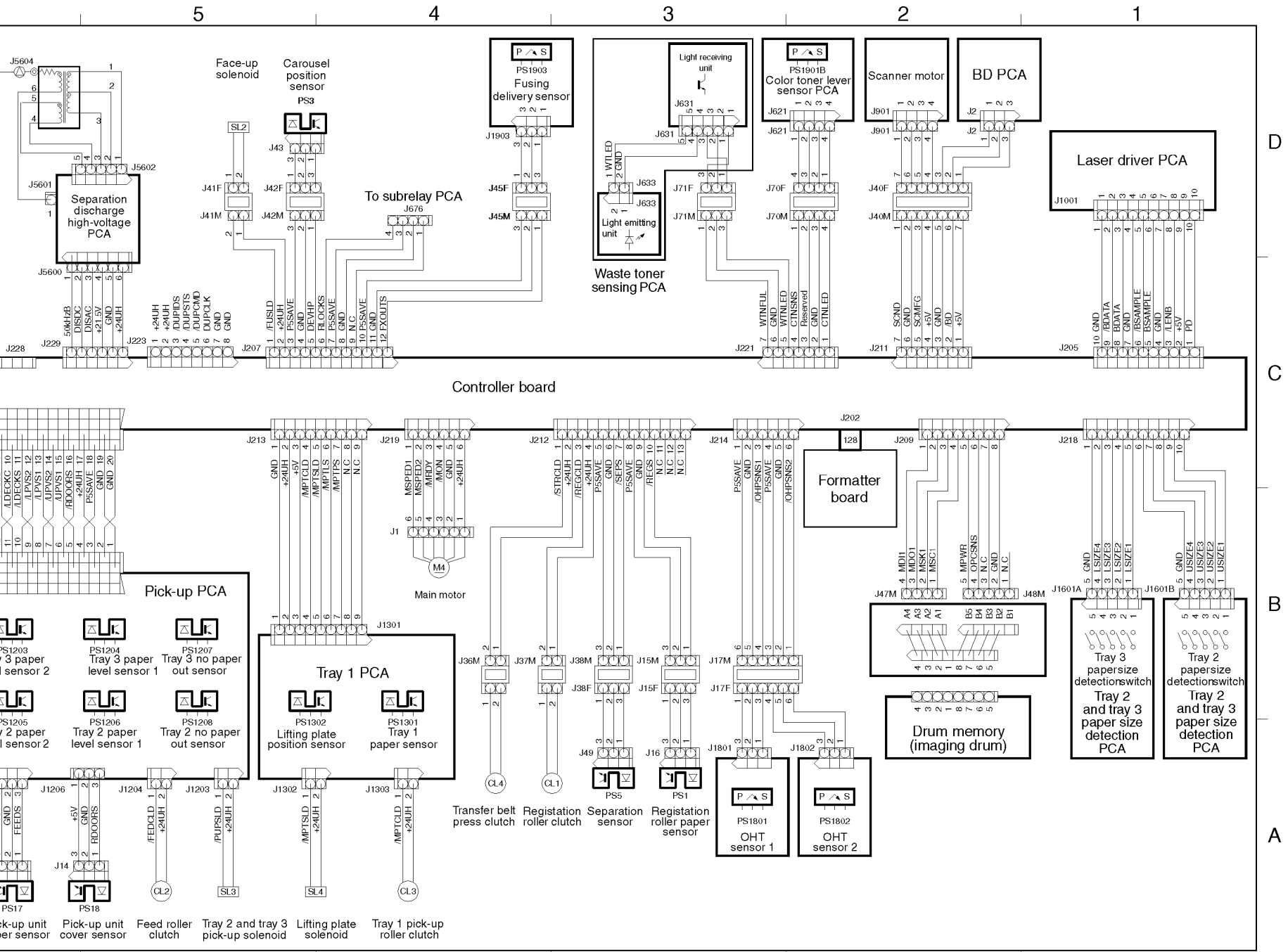
Printer circuit diagram (2 of 2)
