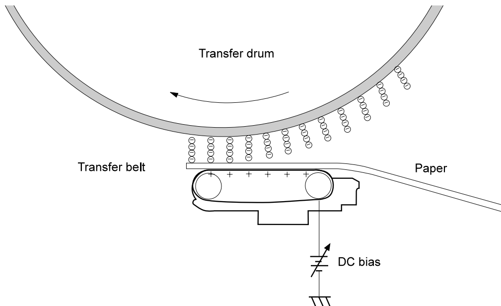
Figure 34. Secondary transfer
