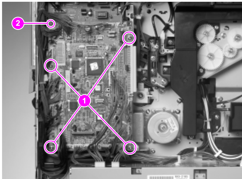
Figure 123. Controller board
